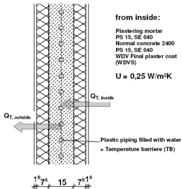
Fig. 2. Schematic diagram of the cross-section of outside walls involved
