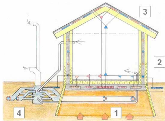
Fig. 1. Schematic diagram absorber- wall- foundation plate
