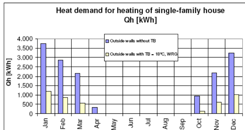
Fig. 2 . Comparison of the conventional construction of a single-family home with the Terra-Sol building technology [1]
