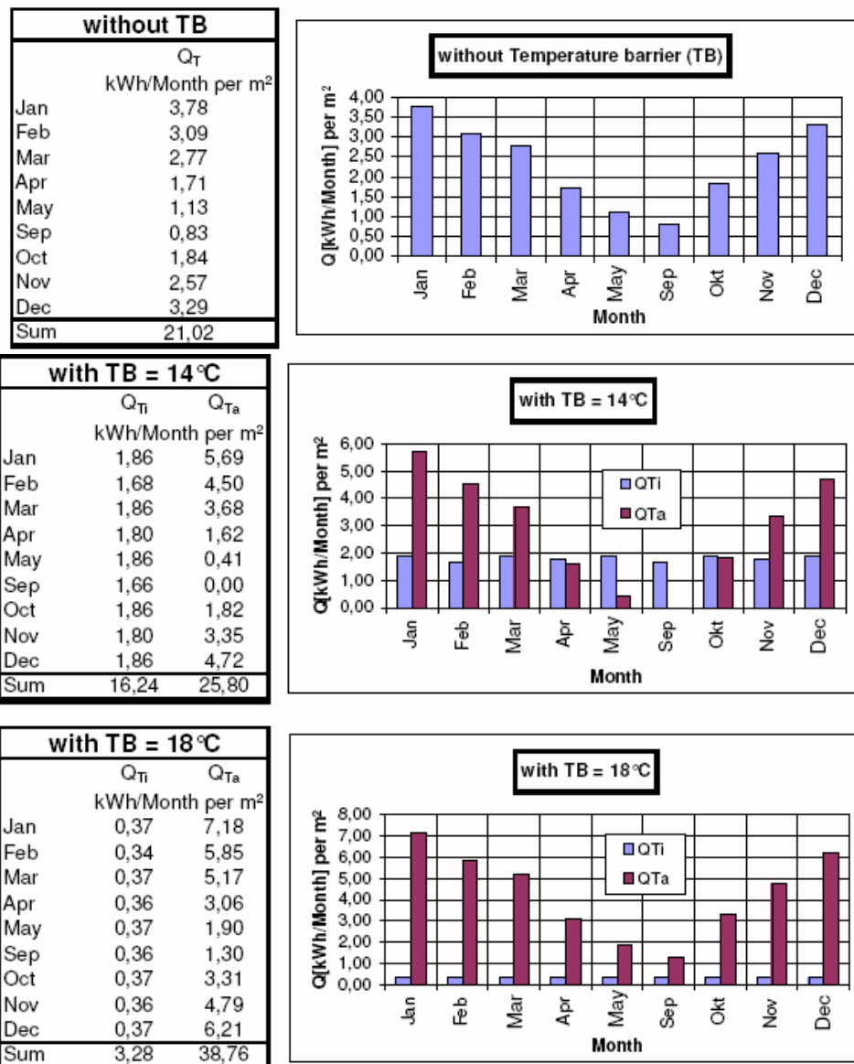
Fig.3. Transmission heat losses of an outside wall without temperature barrier, with temperature barrier = +14^\circ\text{C} and with temperature barrier = +18^\circ\text{C} [1]
